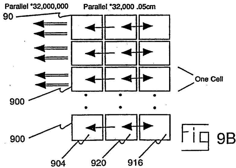
NICE Architecture System (Data Flow)
